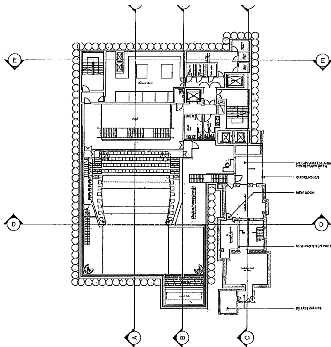
Proposed lower ground floor
