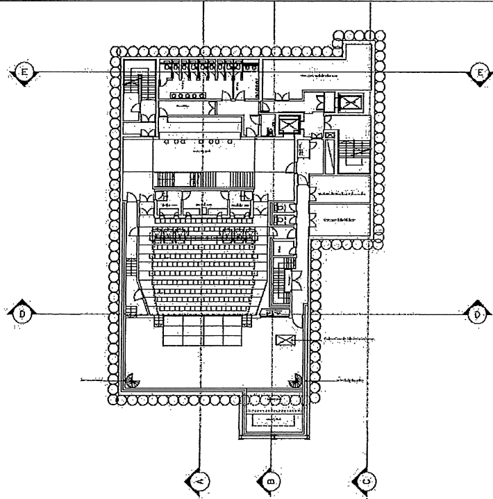
Proposed first basement floor
